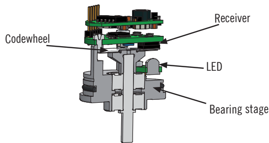
Example of transmissive encoder
