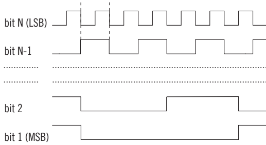
Binary bit parallel output
