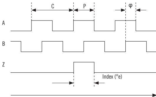
Incremental encoder output signals
