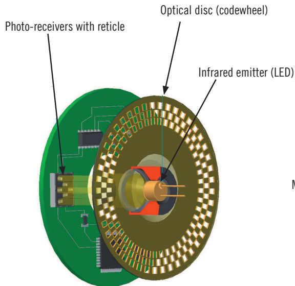
Example of optoelectronic sensor
