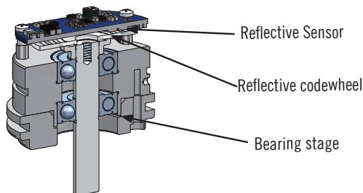
Example of reflective encoder
