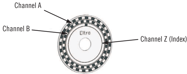
Example of 3 channels incremental encoder codewheel
