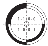
2 Bit optical disc with binary code
