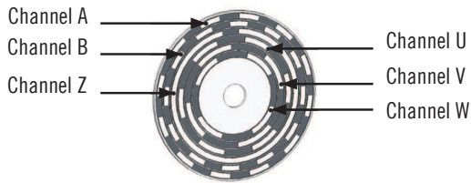
Example of 6 channels commutation encoder codewheel
