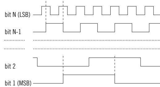
Gray bit parallel output
