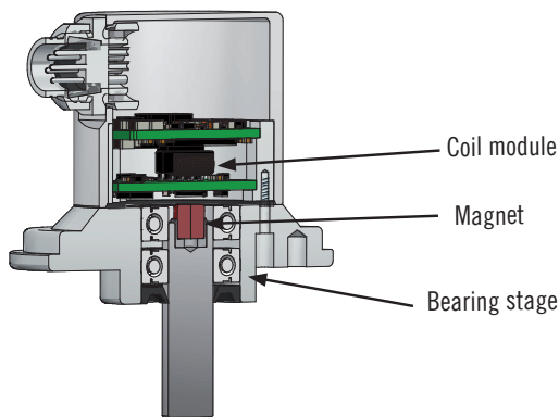
Energy Harvesting engine
