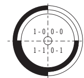
2 Bit optical disc with gray code
