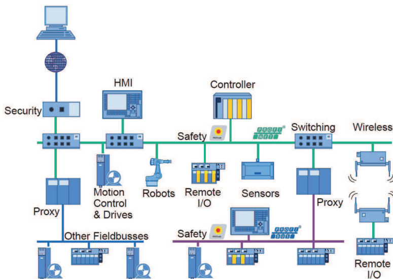
Example of plant network
