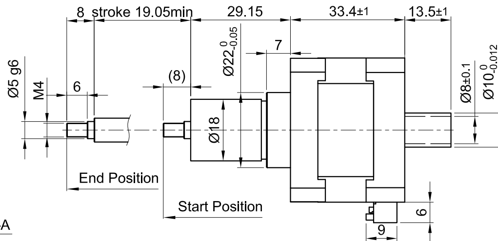
Side view
