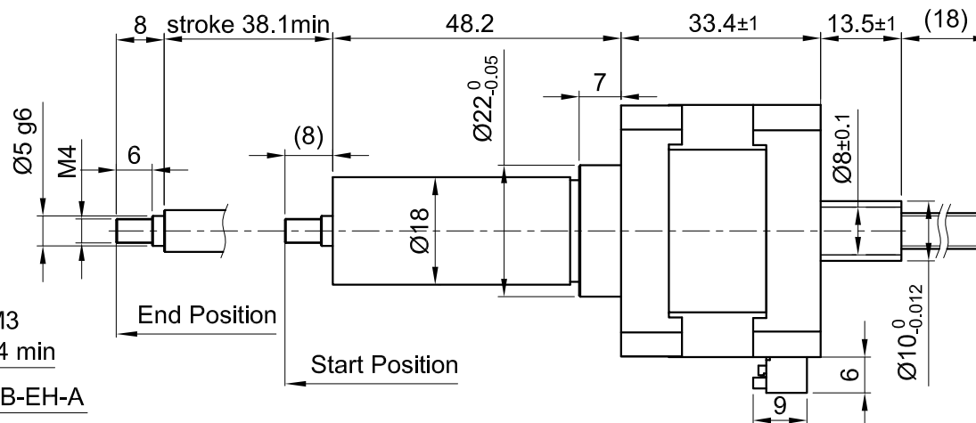
Side view
